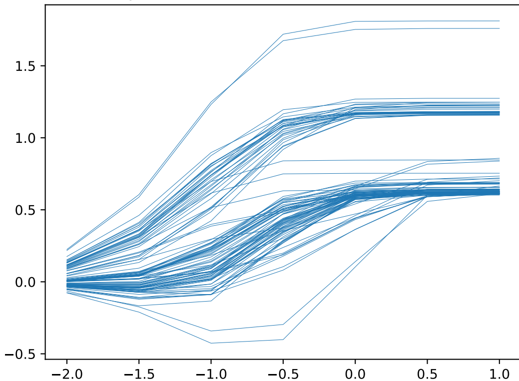
Dynamic Ricci Curvature for Geodesic 0.1
